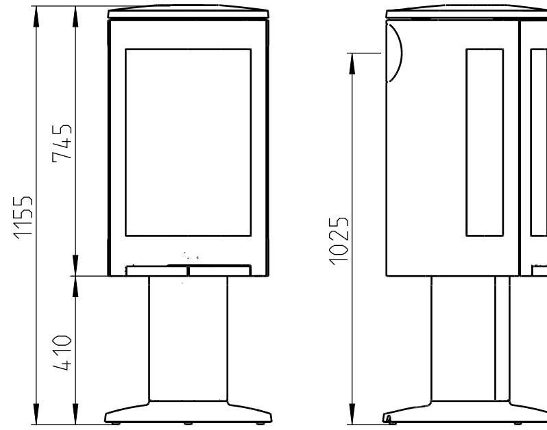
F 373 Advance
