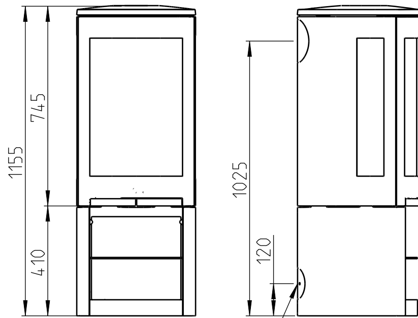
F 371 Advance
